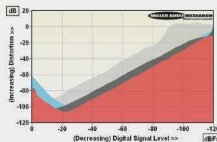
ABOVE: THD vs decreasing digital level at 24-bit/48kHz (1kHz, S/PDIF = red; 20kHz, USB = grey) vs 16-bit CD (1kHz = black, 20kHz = blue)
