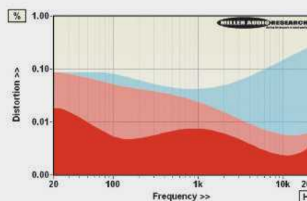
ABOVE: Distortion vs. frequency from 20Hz-20kHz (red, 1V unloaded; shaded, max gain 10mW/25ohm; blue mid-gain)
