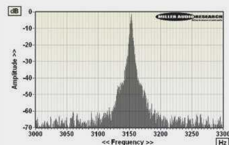
ABOVE: Wow and flutter re. 3150Hz tone at 5cm/sec (plotted \pm 150 Hz, 5Hz per minor division). Some flutter but wow is lower than with RP6
