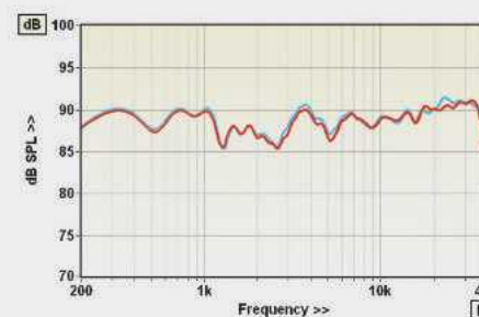
ABOVE: The Olympia III has a slight presence band dip but is essentially flat. Pair matching is excellent
