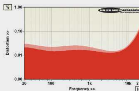
ABOVE: Distortion versus frequency from 20Hz–20kHz (solid red, 1V unloaded; shaded red, 10mW into 25ohm load)
