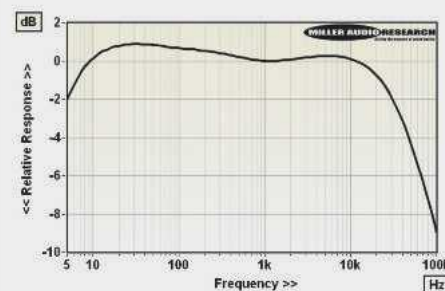
ABOVE: RIAA-corrected frequency response from 5Hz-100kHz (within ±0.9dB from 20Hz-20kHz)
