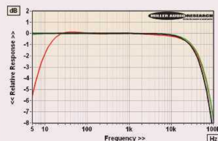
ABOVE: Extended frequency response (5Hz-100kHz) showing CD (black) vs. Aux (green) vs. MM (red)
