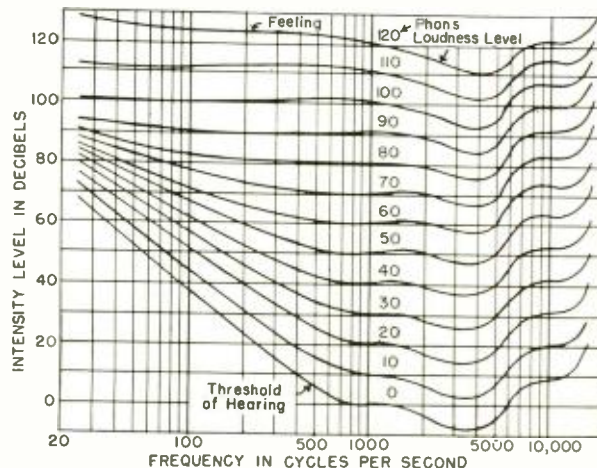
Fig. 2. Contour lines of equal loudness for normal ears (after Fletcher and Munson). 0 db = .000204 bars = 10^{-10} watts per sq. cm. (Courtesy Journal of Acoustical Society of America)
