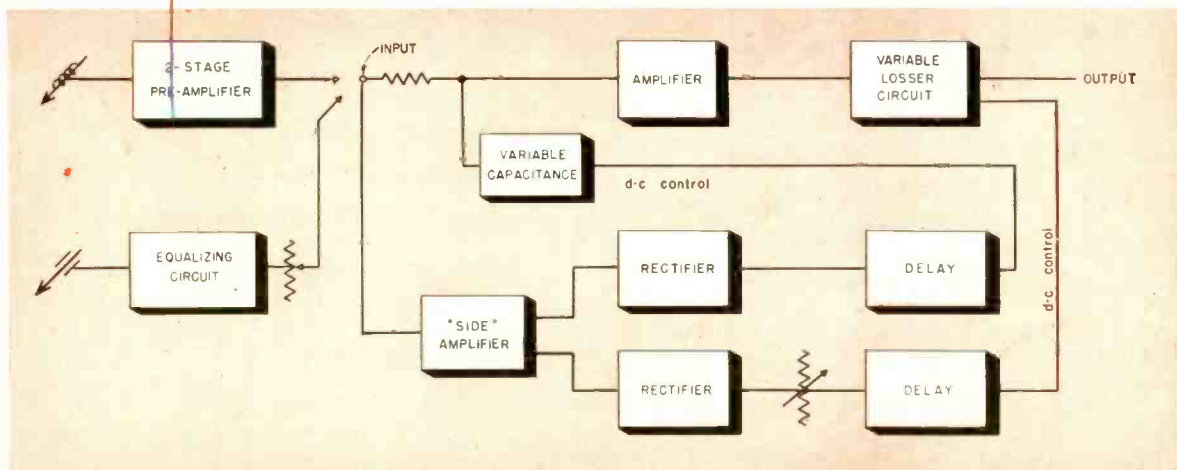
Fig. 1. Block schematic showing arrangement of components for combination scratch suppressor and expander, fed from either a magnetic pickup with a preamplifier, or from a crystal pickup and a potentiometer volume control.
