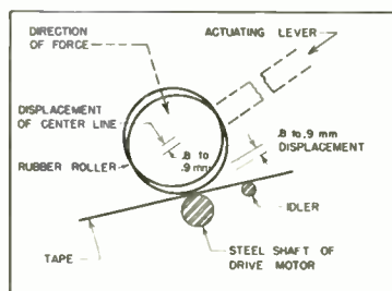
Fig. 8. Detail of tape drive mechanism.
