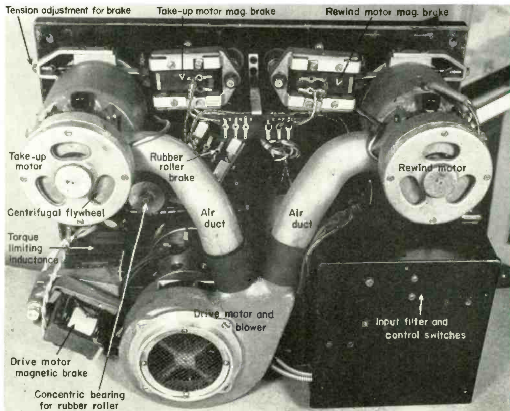
Under-chassis view of the Magnetophon.
