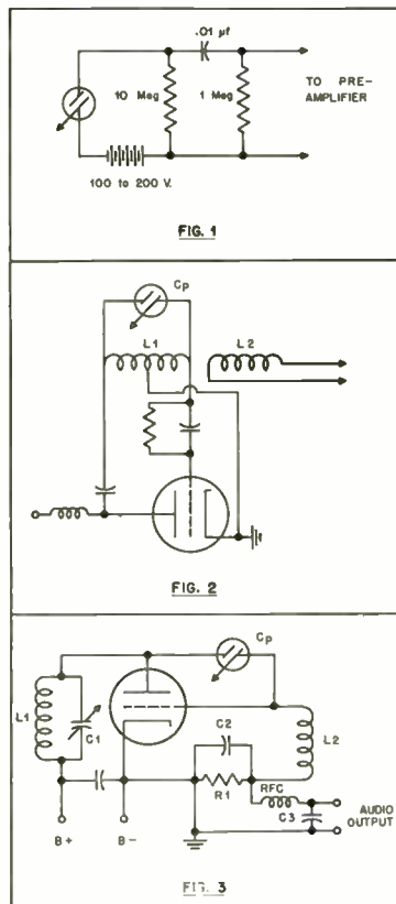
Fig. 1. Early type of capacitive pickup, which was connected like a condenser mike. Fig. 2. Using a capacitive pickup to frequency modulate an oscillator. Fig. 3. Using the capacitive pickup to vary the voltage drop across the resistor R_1 , in accordance with the a-f signal.
