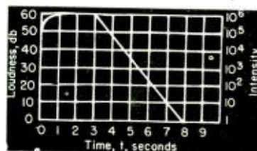
Fig. 2. Logarithmic plot of growth and decay (growth in 1 second, constant 2 seconds, decay in 5 seconds.)
