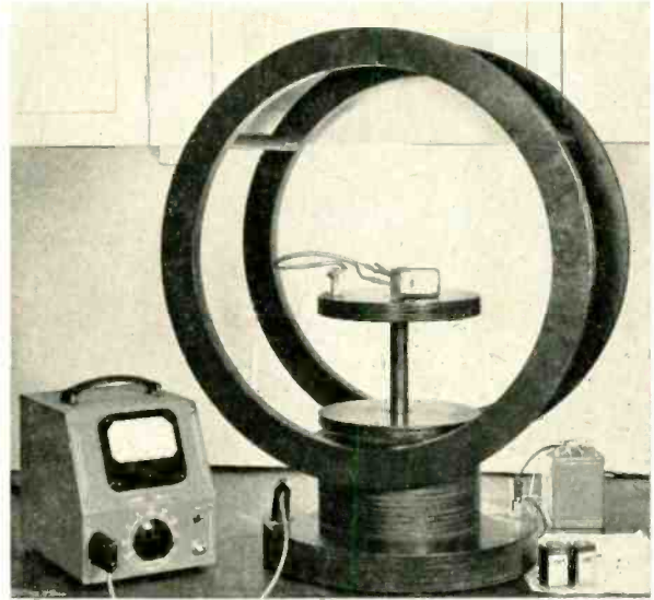
Fig. 3. Equipment used for testing efficiency of transformer shielding.
