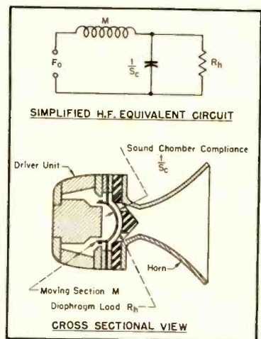
Fig. 1. Compression-type high-frequency unit.
