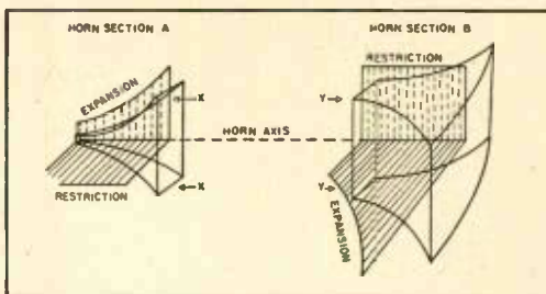
Fig. 5. Flare reversal of the horn walls turns the direction of the wave-front expansion from vertical to horizontal.
