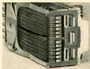
New relays must be able to operate one billion times—equal to once-a-second for 30 years. Employing a sound recorder as a precision vibrator, Bell scientists learned to evaluate the effect of sideways motion on relay life. Such rubbing motion is limited to one-thousandth of an inch in the new relays.
