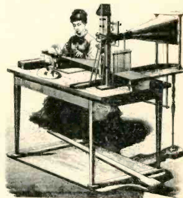
Fig. 7-4. The Faber speech organ. speech could be "played" from the in front of the bellows. From: Zeitschrift für Allgemeine Sprach 1884.
