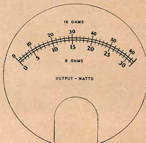
Fig. 2. Meter scale for use on 2-amp. C. E. thermocouple meter with calibrations directly in watts output for 8- and 16-ohm loads.
