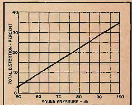
Fig. 13. Harmonic distortion of the human hearing system at 1000 cps. Includes harmonics from second to fifth, inclusive.
