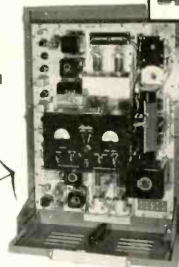
Model 260S Power Supply
