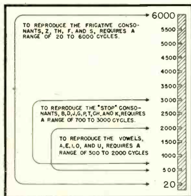
Fig. 2. Frequency range required for intelligible transmission of various speech sounds.
