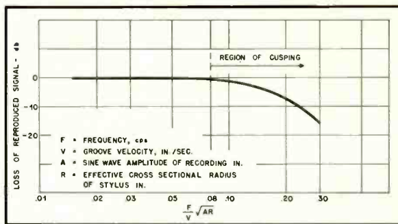
Fig. 4. Effect of frequency response of varying degrees of cusping. This curve may be used for any embossed recording by substituting the correct values for F , V , A , and R .
