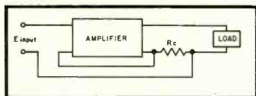
Fig. 12—16. Negative current feedback. The feedback voltage across R_o varies with the current through the load rather than with the voltage across it. Note that an un-bypassed cathode resistor is in exactly the same position in the circuit as R_o above.
