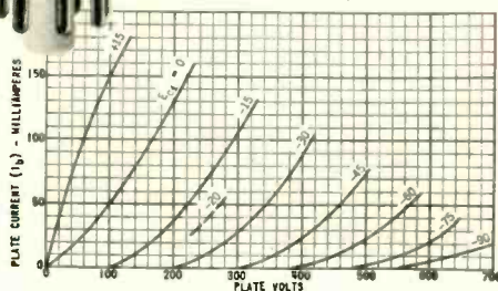
CLASS AB 1 PUSH-PULL AMPLIFIER—TRIODE CONNECTION
