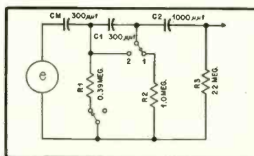
Fig. 10. Low-frequency control circuit.
