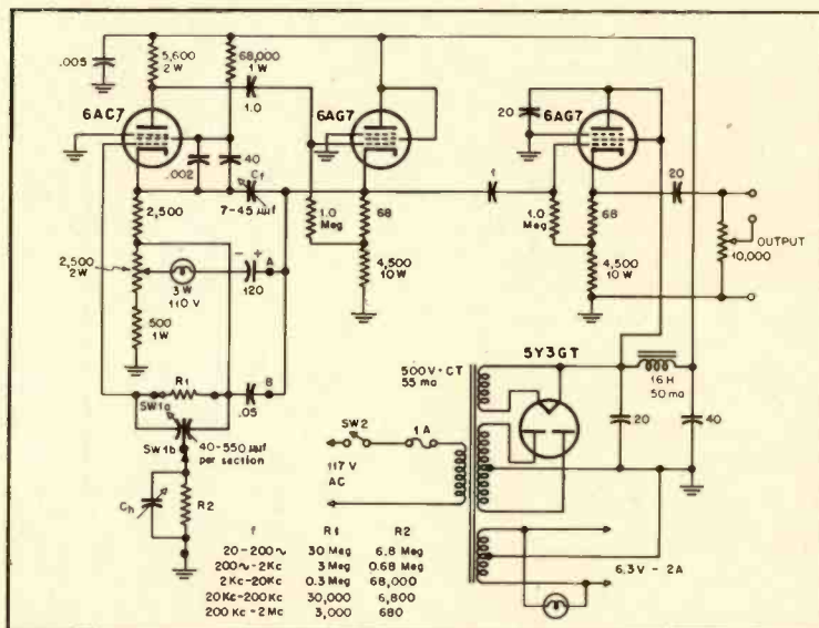
Fig. 3. Complete circuit of practical version of the oscillator and cathode-follower output stage.
