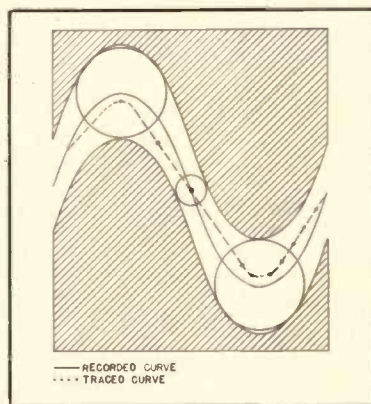
Fig. 9—7. Theoretical (but improbable) tracing distortion. The radius of curvature of the groove modulation is too small for the stylus tip. Note that severe distortion occurs before treble loss becomes significant. (The groove modulation should be shown with a smaller radius of curvature to show the improper stylus fit clear.)
