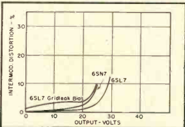
Fig. 9. Distortion measurements on two-stage feedback amplifier of Fig. 2 with 6SN7 and 6SL7.
