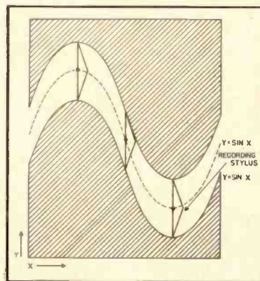
Fig. 9-4. Path of a recording stylus (without burnishing facets) in relation to the groove.
