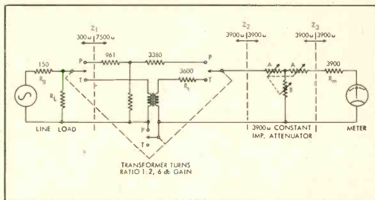
Fig. 6. Method of connecting VU meter to 150-ohm line through matching transformer. Fixed pad is connected at 16-VU point due to power limitations of transformer.
