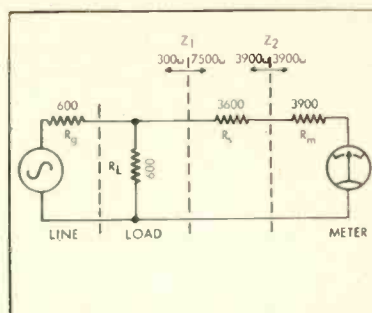
Fig. 4. Basic VU meter circuit. Pointer will indicate zero VU 600-ohm line level of 1.228 volts, which is 4 db above 1 milliwatt.
