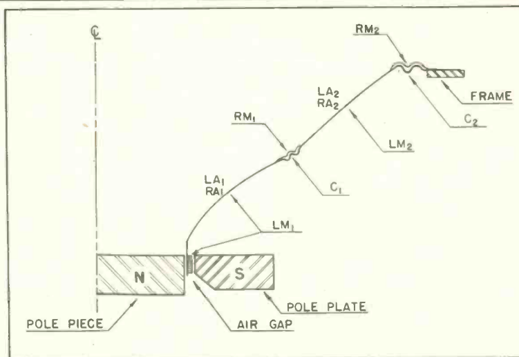
Fig. 4. Double-compliance cone with voice coil in a magnetic air gap. One half of assembly shown.
