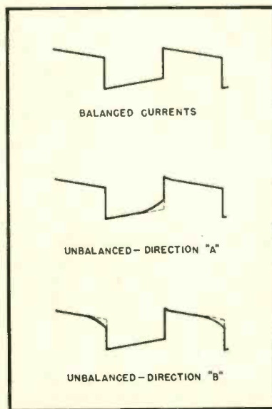
Fig. 11. Effect of current unbalance on square waves. Note that only the low frequency is affected, as indicated by the rounding of trailing edge of wave.
