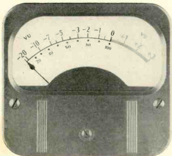
Fig. 1 (left). Type 30 Weston Model 862 VU meter with "A" scale for ease in measuring and testing. Fig. 2 (right). Type 30B meter with predominant percentage modulation scale designed for program line monitoring.
