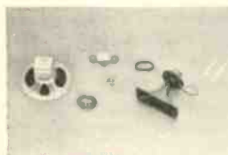
KDU-11 TABLE DUETTE KIT 2-way system. Specially designed for chair side or table TV use. May also be used in 1 1/4 cu. ft. Duette enclosure. Heavy duty 6" x 9" "woofer", compression driver "tweeter", frequency division unit and wiring materials. 3-4 ohms. 20 watts. $23.75
