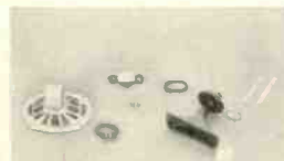
KDU-12 BUDGET DUETTE KIT 2-way system. For maximum results at lowest cost. May be installed in table or 1 1/4 cu. ft. regular Duette or in 2 1/4 cu. ft. Bass-Ultraflex enclosures. 6" x 9" "woofer", direct radiator "tweeter", frequency dividing unit plus wiring materials. 3-4 ohms. 15 watts. $10.50
