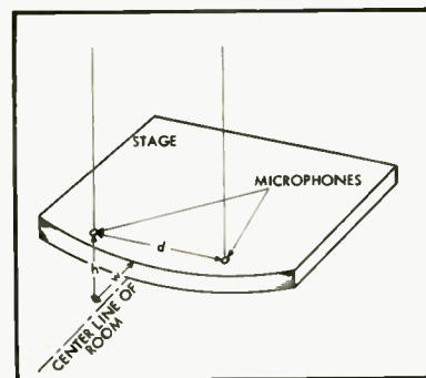
Fig. 5. The three dimensions governing stereophonic microphone placement. The actual dimensions will depend on the size of the pickup area and the factors discussed in the text.
