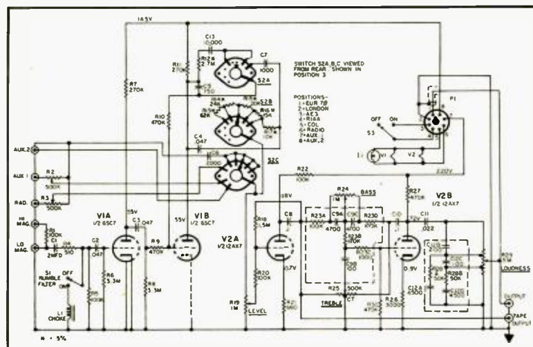
Fig. 3. Schematic of the preamp section of the XA1-320 amplifier.
