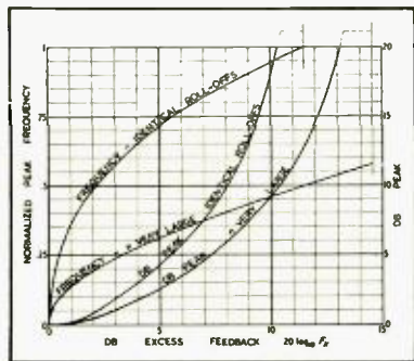
Fig. 16. Limit chart showing the behavior of the four-stage one-and-three case for amounts of feedback causing peaking but not instability. For explanation see Fig. 13.
