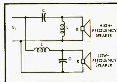
Fig. 1. Typical 12 db/octave constant-resistance crossover network, in the parallel configuration.
