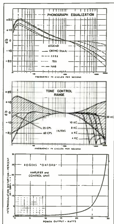
Fig. 6. Performance curves for the "Oxford" amplifier and control unit.
