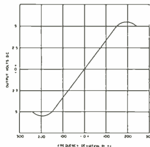
FM discriminator characteristics
