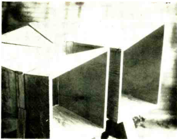
Fig. 1. The semicircular horn before enclosing it in another speaker cabinet. The left orifice is for a 15-in. speaker, tapering to join a 100-sq.-in. throat; the right opening is the mouth of the horn.
