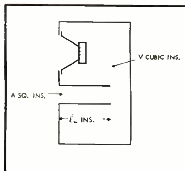
Fig. 4. Parameters important in the design of a ported cabinet.
