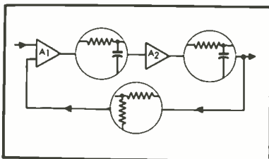
Fig. 5. When single reactance rolloffs are separated by amplifier stages so as not to interact in simple amplification, the addition of feedback causes interaction, and modifies the response in a manner somewhat similar to the circuit of (A) in Fig. 3.
