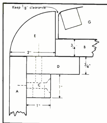
Fig. 13. Detail of front corner construction.
