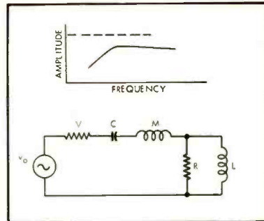
Fig. 5. Velocity-controlled loudspeaker.
