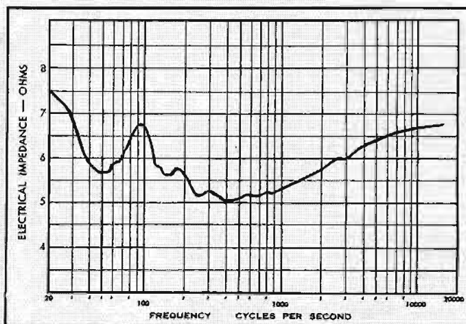
Fig. 2. Electrical impedance of the enclosure with a typical 8-inch speaker.
