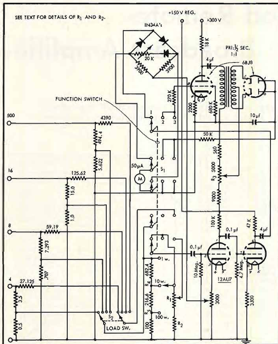
Fig. 3. Complete schematic of direct-reading damping-factor meter.
