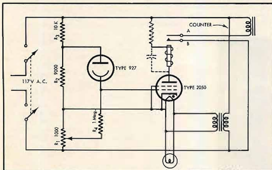
Fig. 1. Complete schematic of photo-relay circuit.
