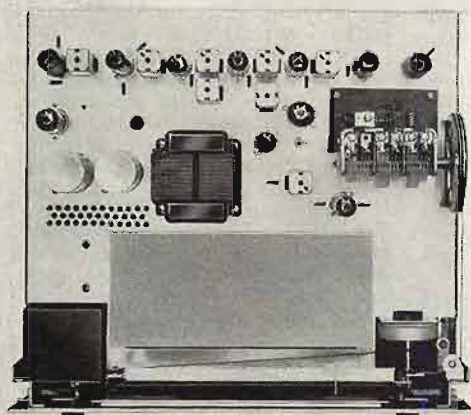
Top view of T250 showing provision for multiplex adapter (MA250)
