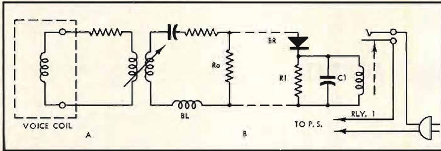
Fig. 4. Feedback-type network to actuate cut-off relay.
