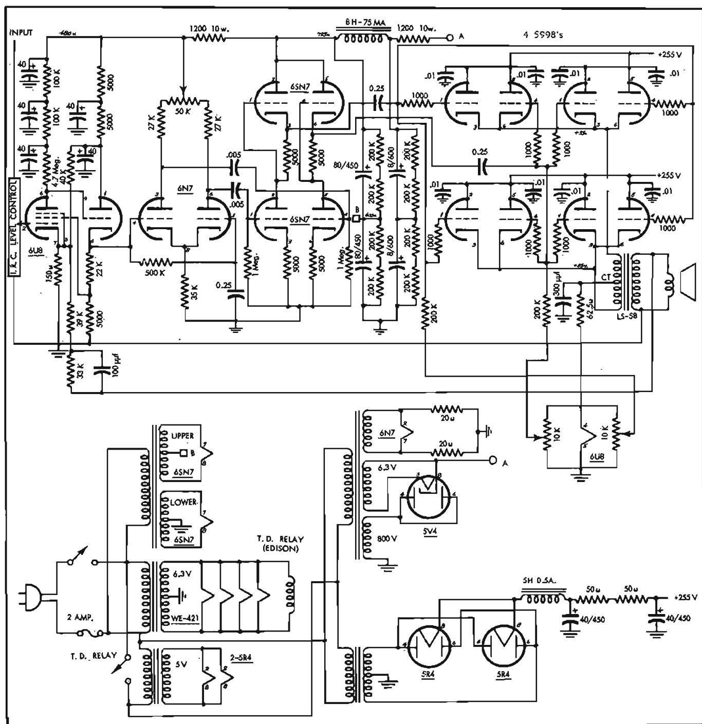
Fig. 1. Complete schematic for the "Purple Cow" amplifier which employs four heavy-duty double triodes in a cathode-follower output stage for reliable and high-quality performance.
