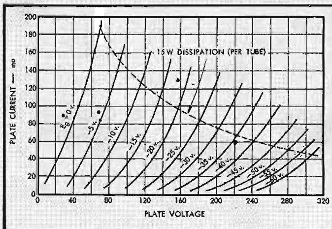
Fig. 3. Plate family for the 5998 tube.
