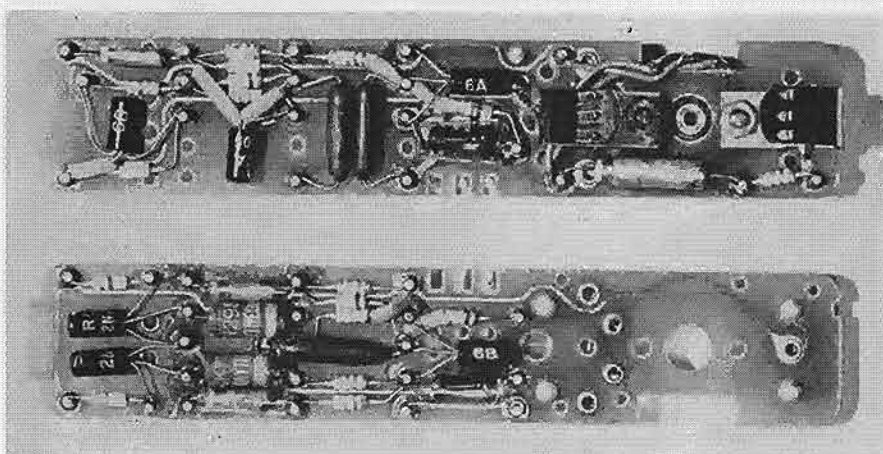
Fig. 7. Details of the two printed-circuit sections which are mounted back to back.
