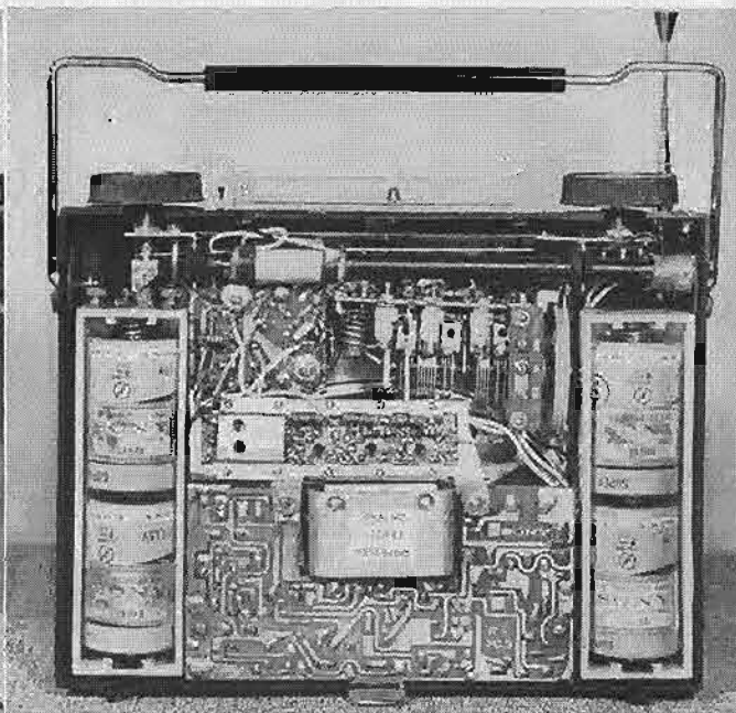
Fig. 1 (left). Sony TFM-151 AM/FM transistorized portable. Fig. 2 (right). Interior of 15-transistor receiver. Note speaker magnet frame projecting through opening in printed-circuit panel.
