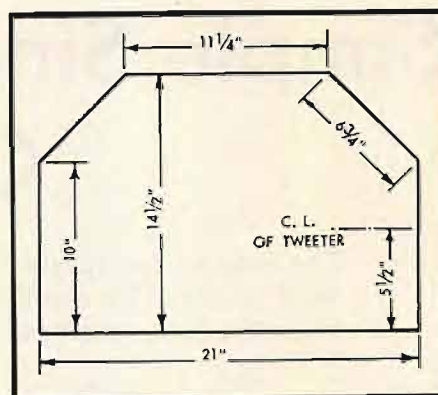
Fig. 2. Physical measurements of the Rebel IV enclosure.
