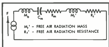
Fig. 6. Equivalent circuit of speaker mechanism in free air.
