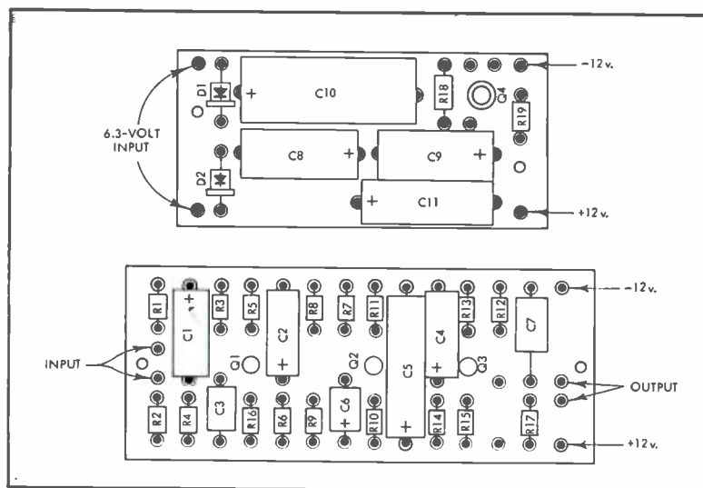
Fig. 4. Ports placement on preamplifier "chassis" (above) and power supply (below).
