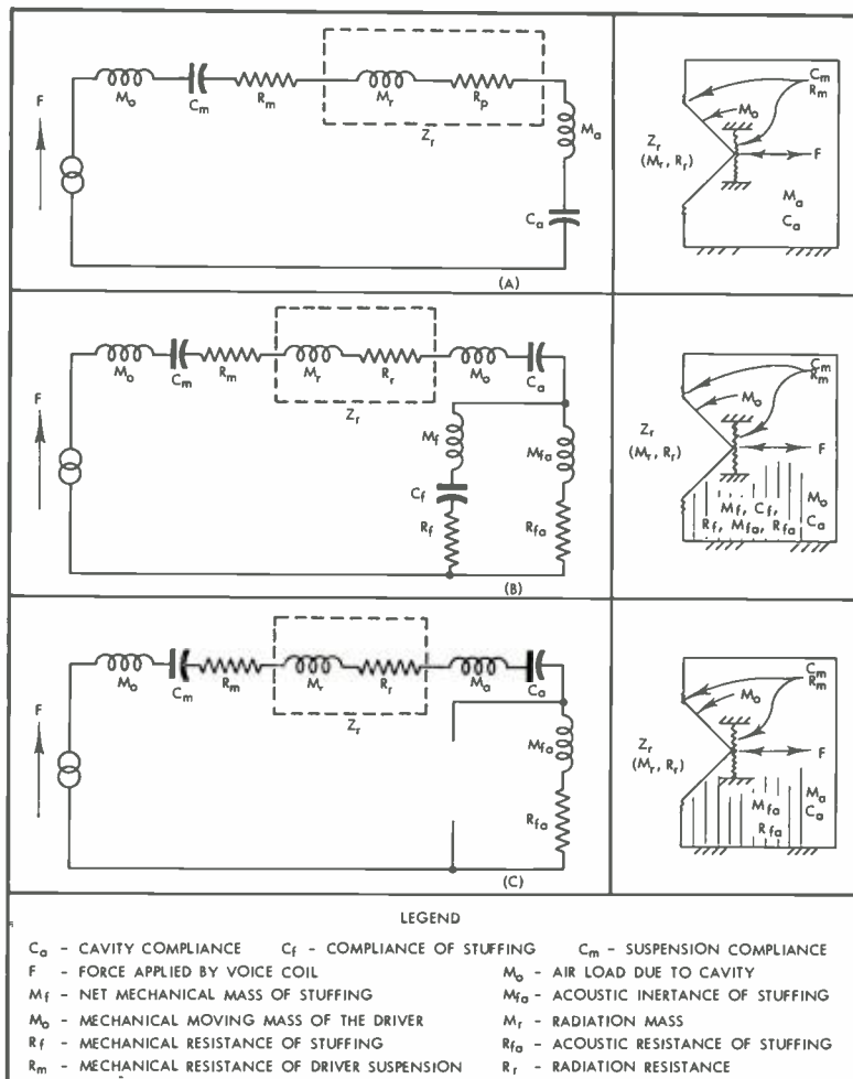
Fig. 3. Equivalent circuits: (A) unstuffed cavity, (B) stuffing placed in cavity loosely, and (C) stuffing placed in holding frame in cavity.
