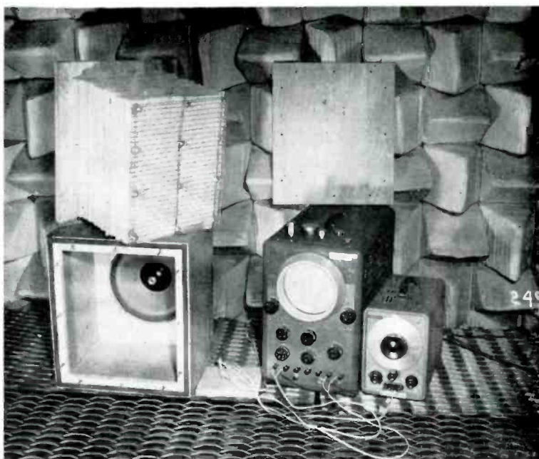
Fig. 4. Experimental apparatus showing inside of enclosure, placement of an additional mass, and the framework for holding the fiberglass stuffing.
