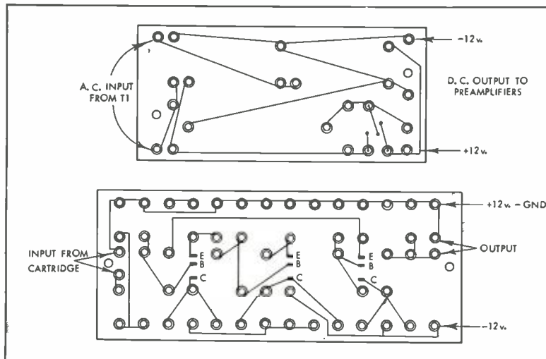
Fig. 5. Underside of preamp and power supply modules showing strapping between eyelets.
