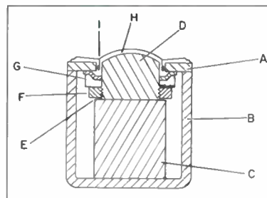
Fig. 3. Cross section of the omnidirectional unit.
