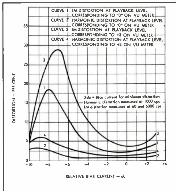
Fig. 8. Variation of tape distortion with changes in bias current.
