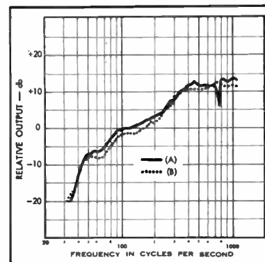
Fig. 8. Axis frequency response curves for direct-radiator closed-box loudspeaker with a 1.5-cu. ft. cavity: (A) empty, and (B) filled with loose fiberglass.
