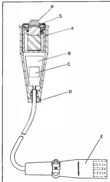
Fig. 8. Cross section of the lavalier microphone.
