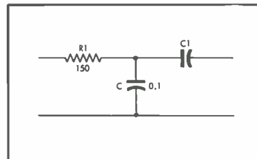
Fig. 9. R_2 of Fig. 1 is replaced by the 0.1- \mu\text{f} capacitor.
