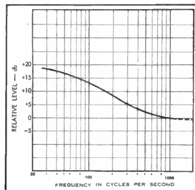
Fig. 2. Low frequency compensation for RIAA characteristic.
