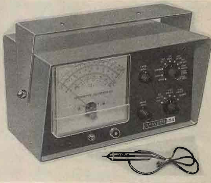
Fig. 5. Lafayette VTVM, Model KT-174.
