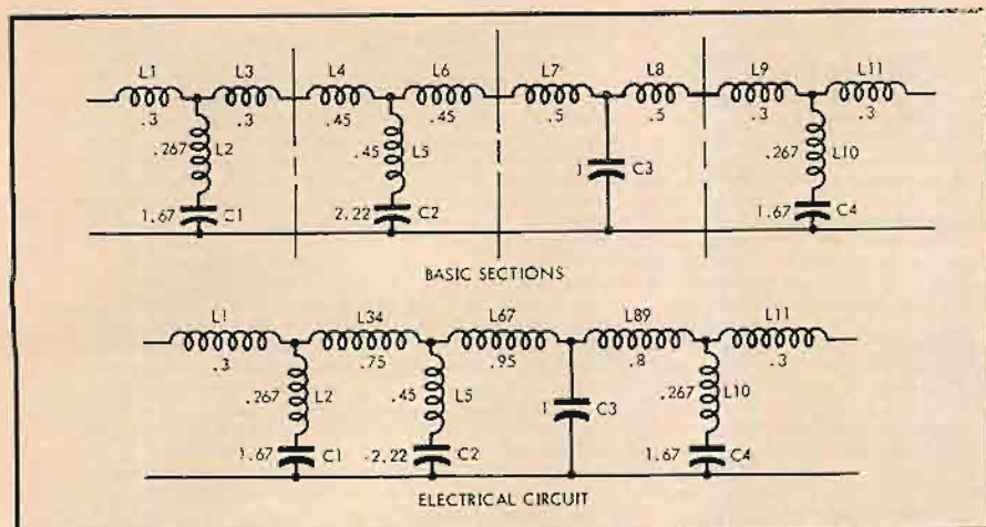
Fig. 5. Electrical derivation of the filter that was an early subject for experimentation in the use of leakage inductance.
