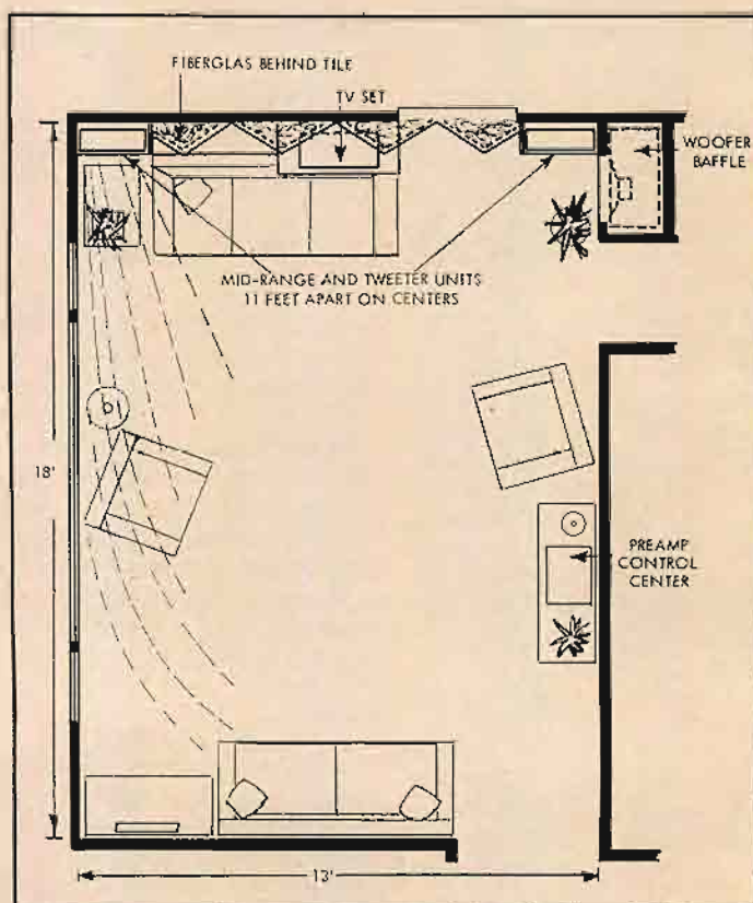
Fig. 4. Floor plan of the listening room.
