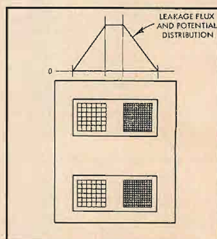
Fig. 2. The geometry of leakage flux through the windows (see text).
