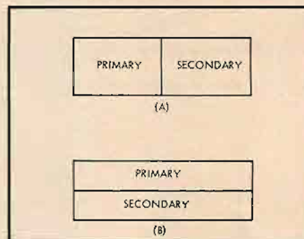
Fig. 3. Two simple ways of arranging windings in standard window shape makes leakage inductance change in ratio 9:1.
