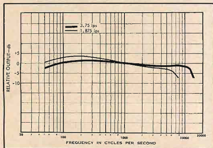
Fig. 3. Record-playback response at 3.75 and 1.875 ips.
