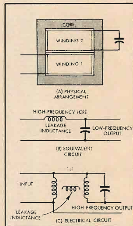
Fig. 7. Derivation of simple high-pass filter using leakage inductance.
