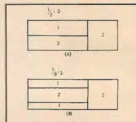
Fig. 4. Two arrangements for combination of tight and loose coupling between different windings (see text).
