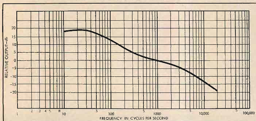
Fig. 7. Frequency response.
